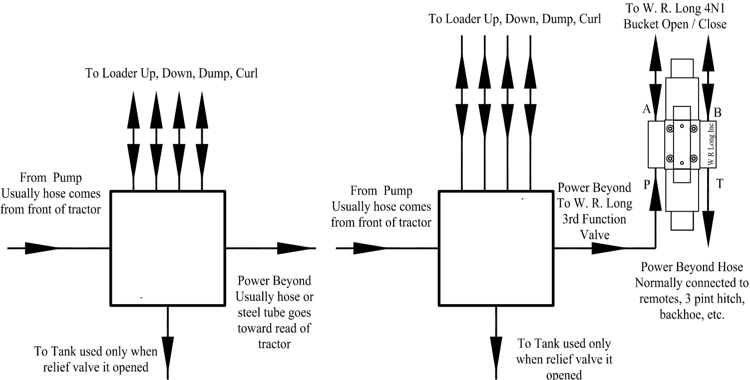
Standard Loader Valve Configuration with W. R. Long Valve Kit Installed
