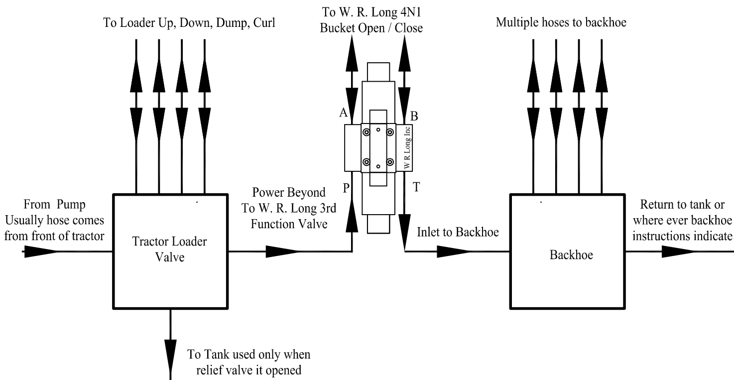
Standard Loader Valve Configuration with W. R. Long Valve Kit Installed with Backhoe
